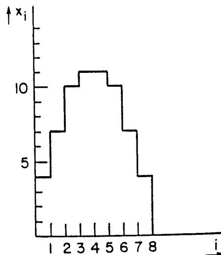
Fig.4. Segment histogram for a 64-bit adder: m=8
