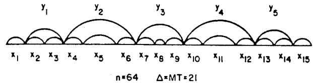
Fig.7. Carry chain of a 64-bit adder: MT = 21
