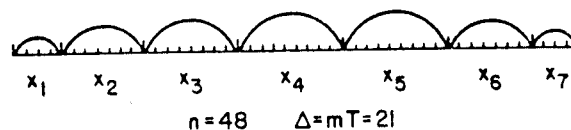
Fig.3. Carry chain of a 48-bit adder: n=48 , mT=21
