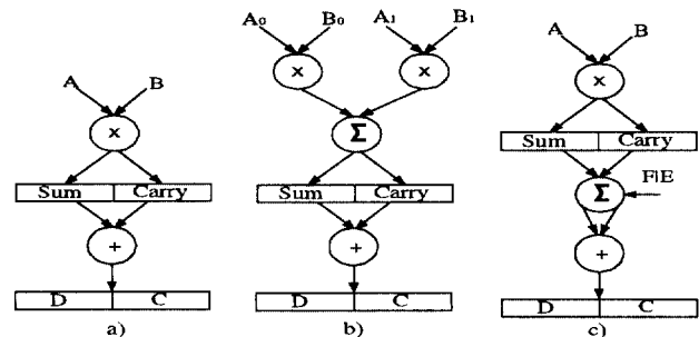
Fig. 4. Two cycle multiply operation a) 8x8 or 16x16, and b) 24x24 or 32x32, and c) multiply accumulate operation.
