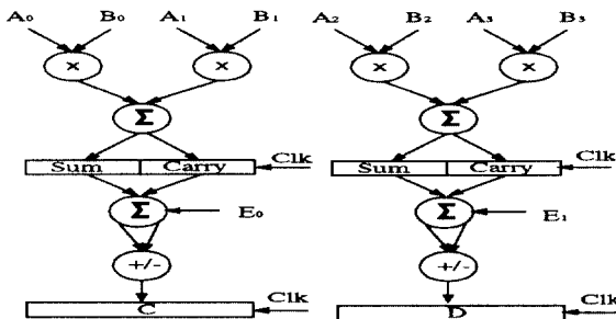
Fig. 2. Macro-level implementation of the datapath.
