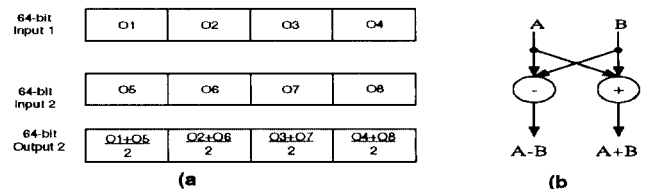
Fig. 3. a) Parallel averaging operation, b) Butterfly Operation on A and B.
