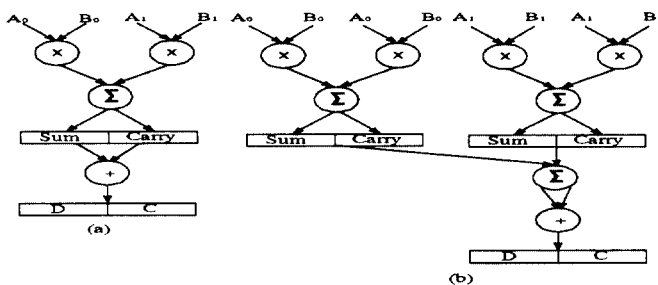
Fig. 5. Sum of two products: (a) Byte or half-word, and (b) 32x32.
