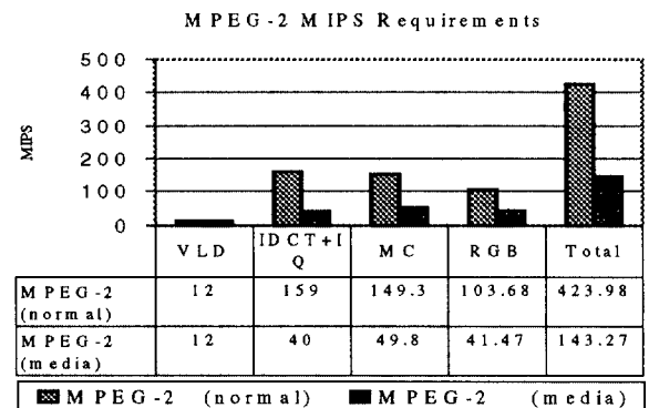
Fig. 1. MPEG-2 MP@ML execution profile with and without media instructions.
